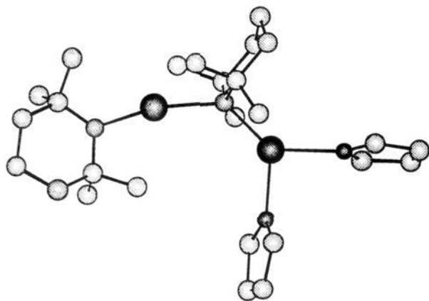
Figure 3. Optimized structure of the (THF) 2 -solvated LiTMP open dimer 32 . Hydrogen atoms have been omitted for clarity.
